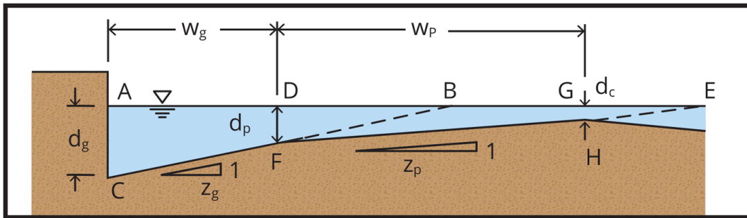
(a) Gutter and Roadway Profile with Vertical Kerb
