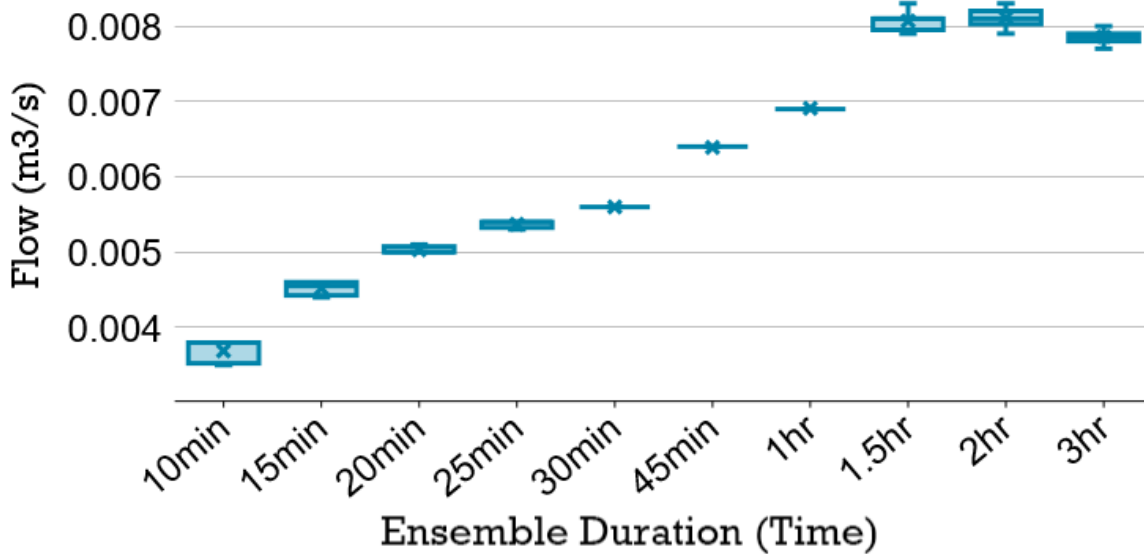
Figure 9.6.32. Peak flows from the Basin for 50% AEP Events
